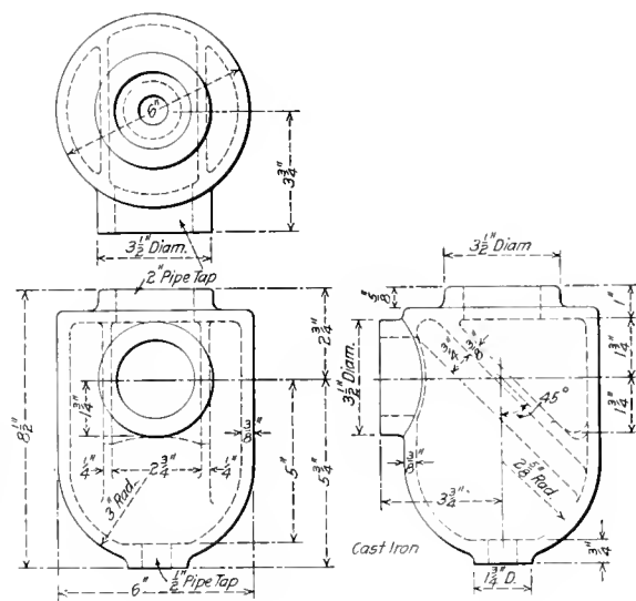
Exhaust Steam Separator for Headlight Service
